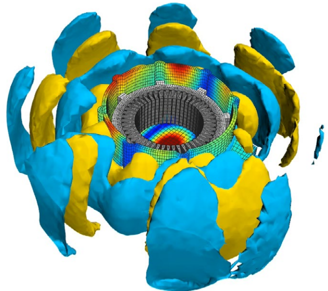
Pressure field generated by an electric motor, whose vibration was calculated by MSC Nastran
