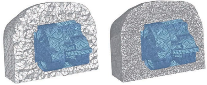
Adaptive meshing: automatic mesh generation optimized for specific computational frequencies
