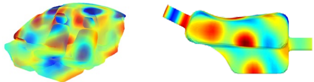
Acoustic mode of an air cavity
