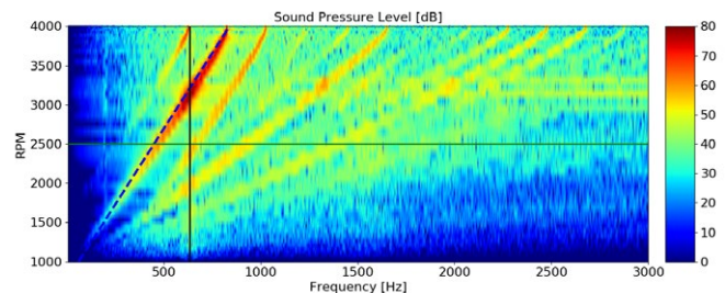
Waterfall diagram of the sound pressure level as a function of frequency and engine RPM
