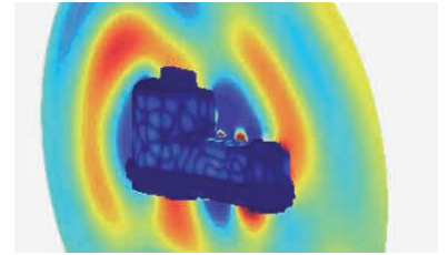
Sound radiation by a vibrating gearbox solved by DGM
