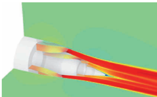
Acoustic propagation from aircraft engine exhaust
