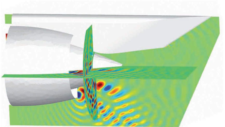
Complex propagation of a high order duct mode through the exhaust of an aircraft jet engine
