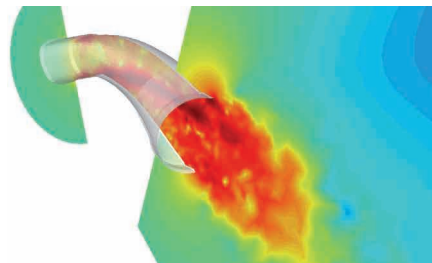
Sound pressure level of air conditioning duct. Correlation between Actran AeroAcoustics predictions and measurements.
