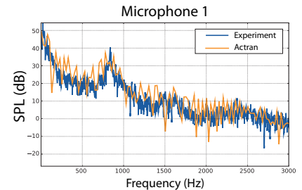
Sound pressure level of air conditioning duct. Correlation between Actran AeroAcoustics predictions and measurements.
