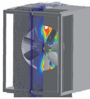
Fan noise application. Correlation between Actran AeroAcoustics predictions and measurements.
