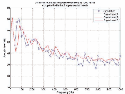
Fan noise application. Correlation between Actran AeroAcoustics predictions and measurements.
